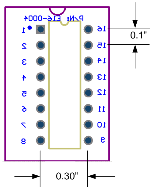
Bottom Side (Top View X-Ray)
